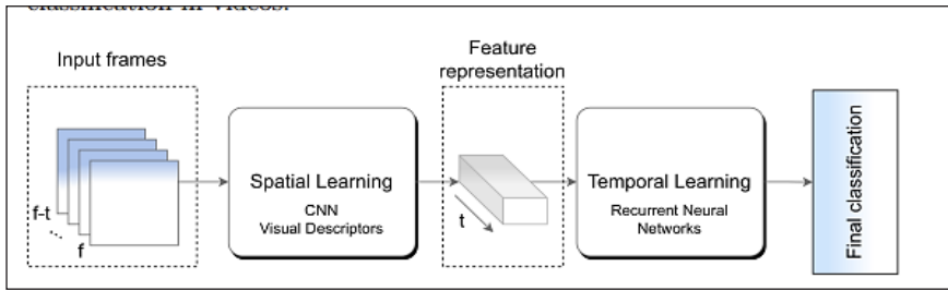
Figure (1) diagram of neural networks architectures [3].
