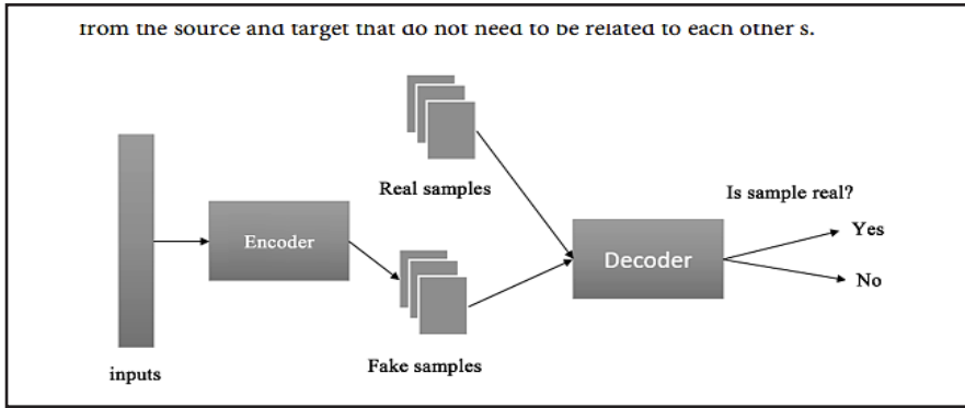
Figure (4) GNA architecture (Pouyanfar, S., et al., 2018)
